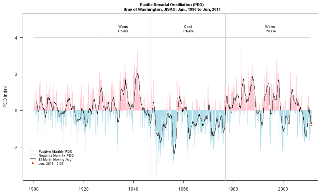
FIGURE 4.4 - THE PACIFIC DECADAL OSCILLATION (PDO)
