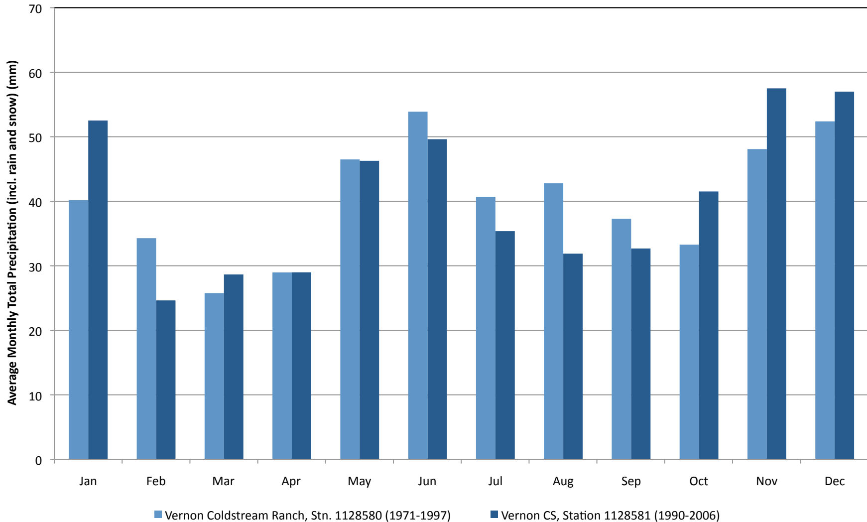
Figure 4.1 Historical Average Monthly Total Precipitation in Vernon
