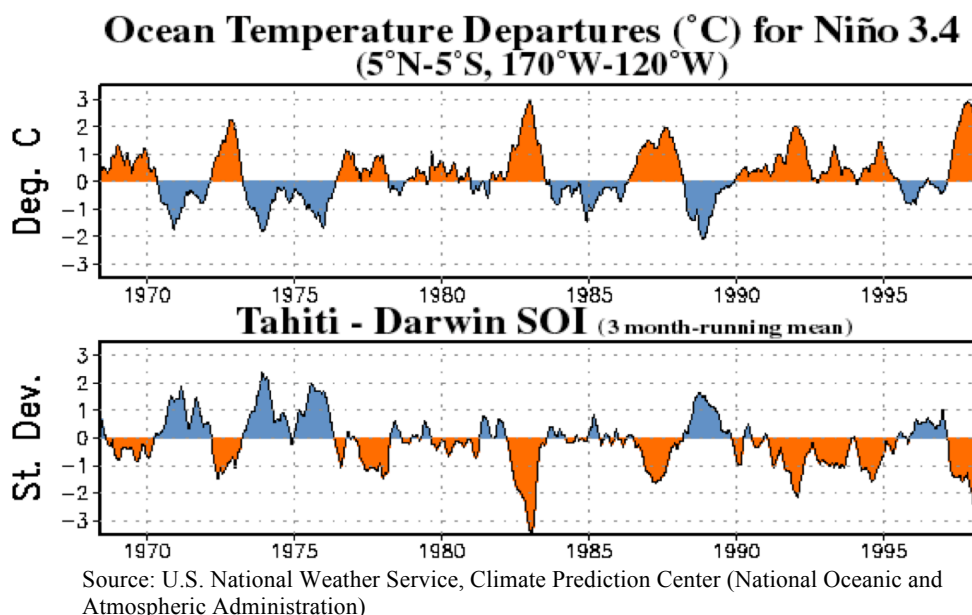
FIGURE 4.3 - THE SOUTHERN OSCILLATION INDEX (SOI)
